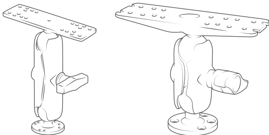
C Size 1.5" Ball Mounts Holds up to 4 lbs 4"–7" Fishfinders & Plotters
